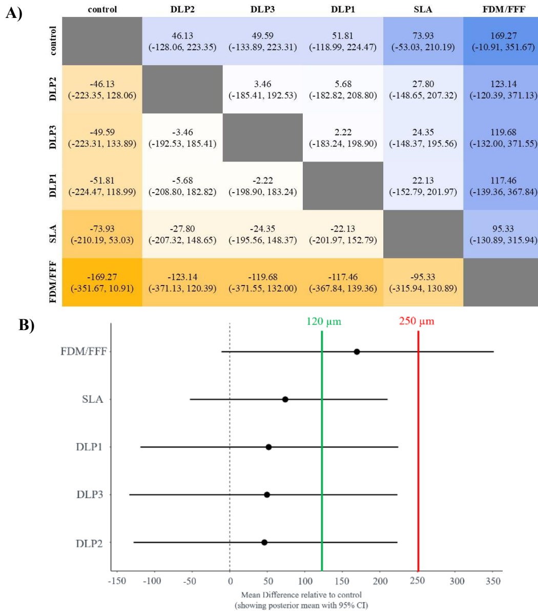
Figure 7. The mean difference of Trueness deviation at arch level using layer thickness over 50 \mu\text{m}
